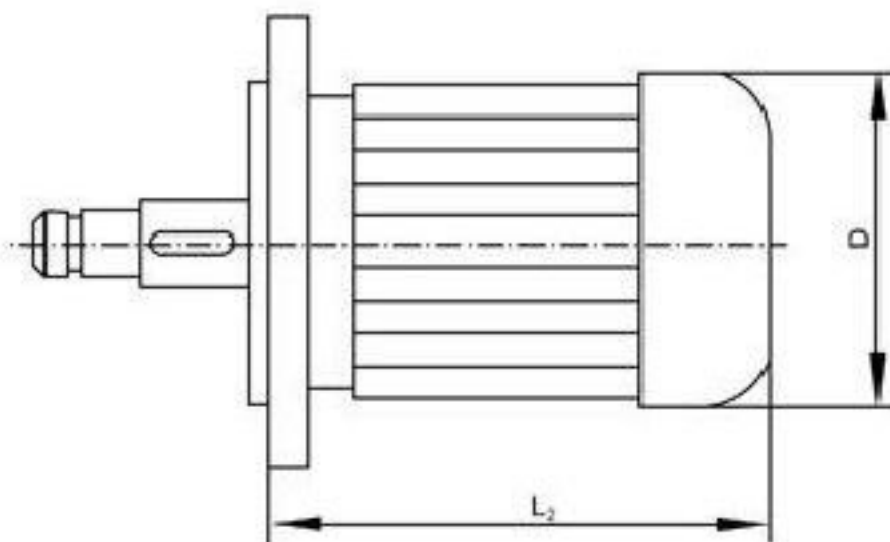
十、WB 系列减速机常用电机及电机外型尺寸一览表 Common motors for WB series of speed reducers and motor appearance size table
