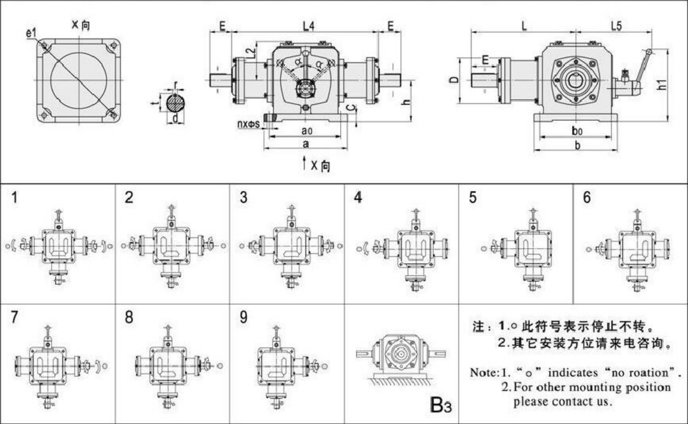
尺寸图表、轴配置及轴旋转方向的关系、安装方位： The relationship between shaft arrangements and direction of shaft rotation, Mounting position and dimension sheets:
