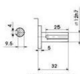
Detailed gearbox output shaft dimension
