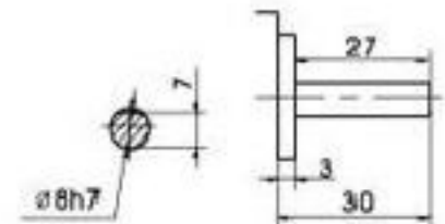
齿轮箱输出轴详细尺寸 Detailed gearbox output shaft dimension
